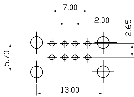
TOP VIEW PCB LAYOUT RECOMMENDED
